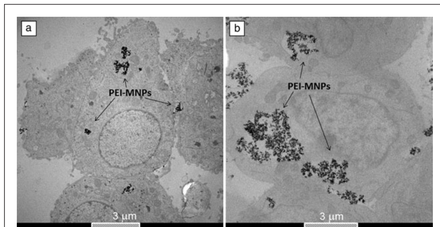
Figure 1. Typical transmission electron microscope images of (a) PC12 and (b) SH-SY5Y cells incubated with polyethyleneimine (PEI)-coated magnetic nanoparticles (MNPs) of 25 nm size. The different amounts of MNP uptake are a characteristic of each neural cell type.
