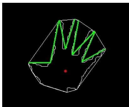
Figure 6. Convexity defects.
